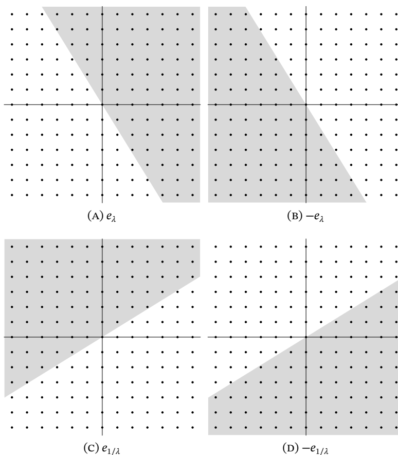
FIGURE 5.2. The four positive cones (shaded) in the example of the figure eight knot complement.
