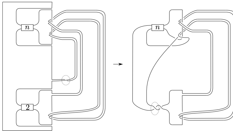
FIGURE 9. The deformation for K_2 . Let \ell be the right link.
