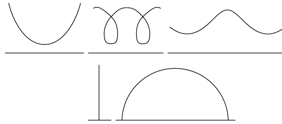
Figure 5. Smooth regions of the cluster are parts of Delaunay hypersurfaces: Catenoid, nodoid, unduloid, vertical plane, sphere.
