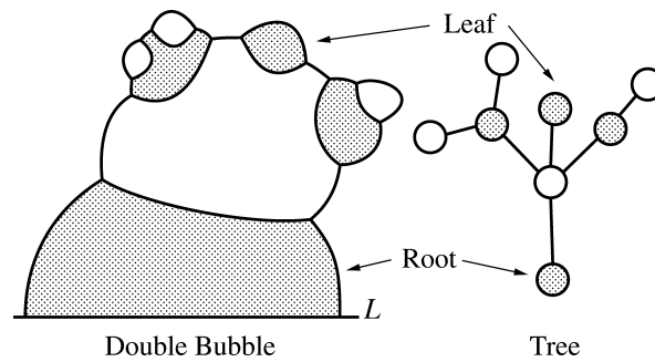
Figure 4. A nonstandard minimal double bubble must be a hypersurface of revolution consisting of a central bubble with layers of toroidal bands. Here we show the generating curves of a typical 4+4 double bubble, together with the associated tree T .
