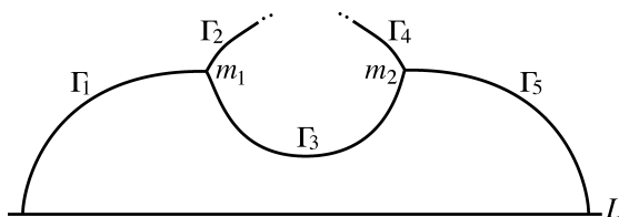
Figure 10. A root involves five arcs: \Gamma_2 , \Gamma_3 , \Gamma_4 , and the two circular caps \Gamma_1 and \Gamma_5 . In general, each vertex can be rotated m_i notches counterclockwise from the pictured configuration, in which all arcs are graphs and m_1 = m_2 = 0 .
