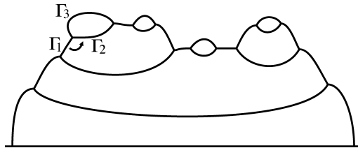
Figure 7. From the curves of Figure 6, vertex v_{123} \equiv \bar{\Gamma}_1 \cap \bar{\Gamma}_2 \cap \bar{\Gamma}_3 has turned one counterclockwise “notch,” since \Gamma_3 has passed the vertical. Hence m = 1 for v_{123} .
