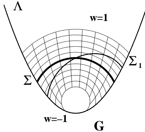
Figure 1. Example of curvilinear coordinates.
