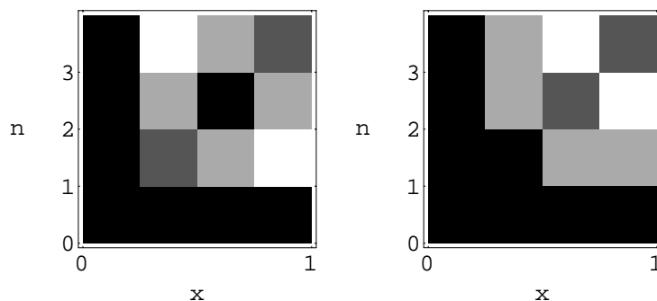
Figure 1. z_{4,\text{id}}\text{wal}_n, n = 0, 1, 2, 3 and z_{4,\varphi}\text{wal}_n, n = 0, 1, 2, 3 .
