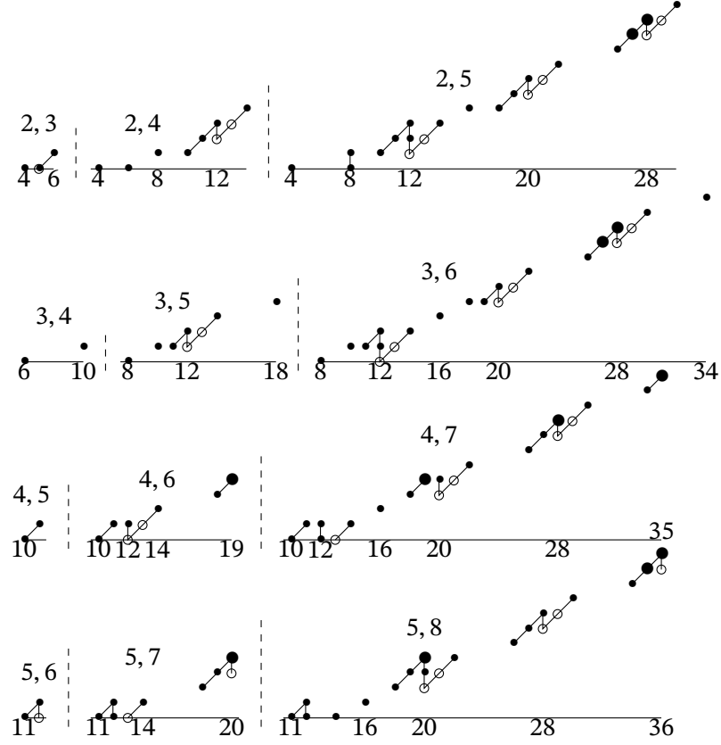
Figure 4.11. \mathcal{E}'_{e,\ell} and differentials
