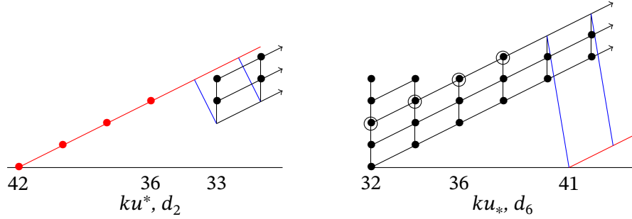
Figure 9.10. Duality of a d^2 and d_6 differential.
