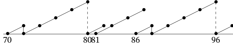
Figure 5.1. B_{3,4} \subset ku_*(K_2)
