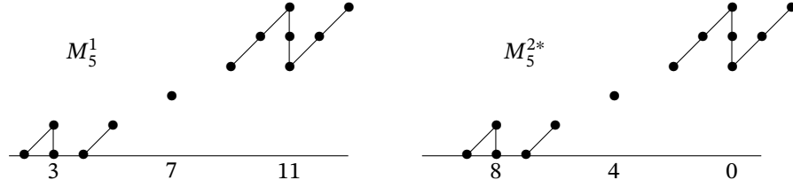
Figure 19.2. Dual M_5 's.
