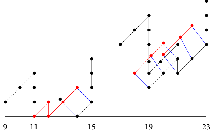
Figure 13.4. Figure 13.1 after replacement
