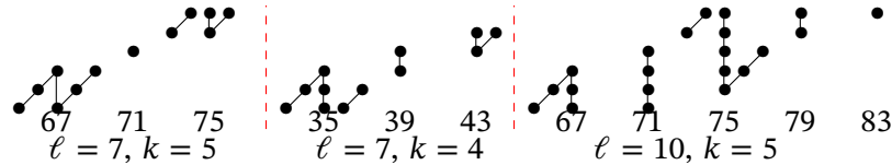
Figure 5.8. Examples of Theorem 5.5(1)
