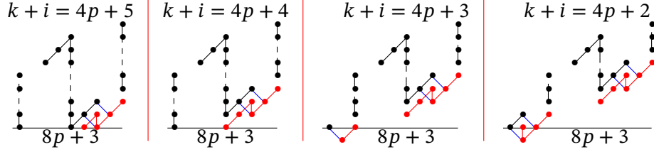
Figure 13.7. M_k^i + \Sigma^2 \widehat{M}_4^{k+i-4}
