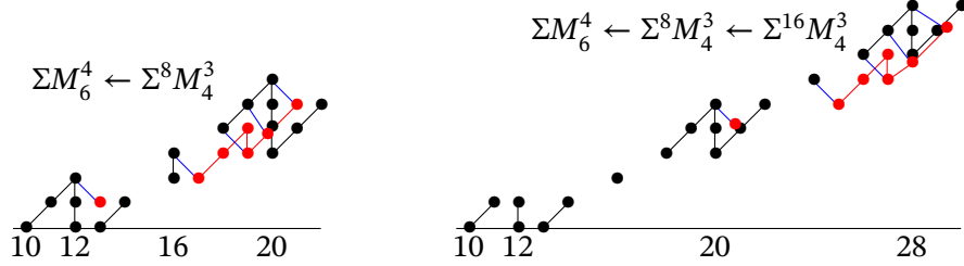
Figure 13.9. First two arrows of (13.3)
