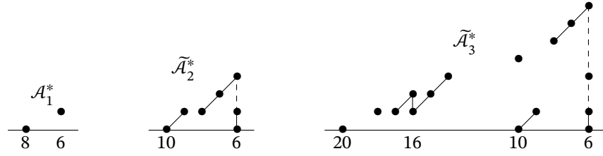
Figure 18.6. Charts for k \leq 3
