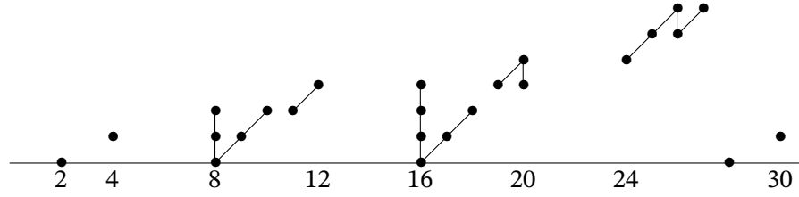
Figure 3.1. \mathcal{A}_1, \mathcal{A}_2 , and \mathcal{A}_3
