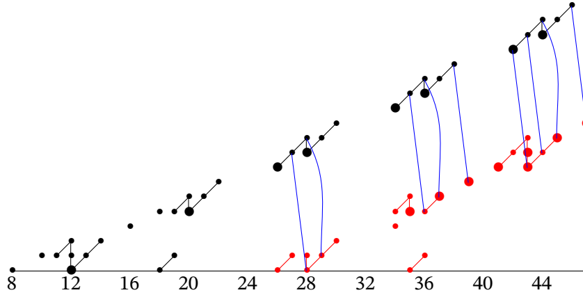
Figure 14.7. Forming the result of (14.5)
