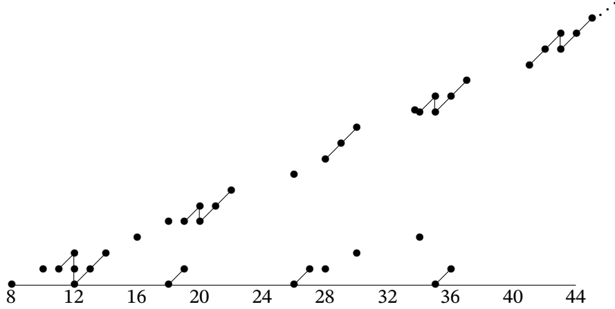
Figure 14.8. Final result of (14.5)
