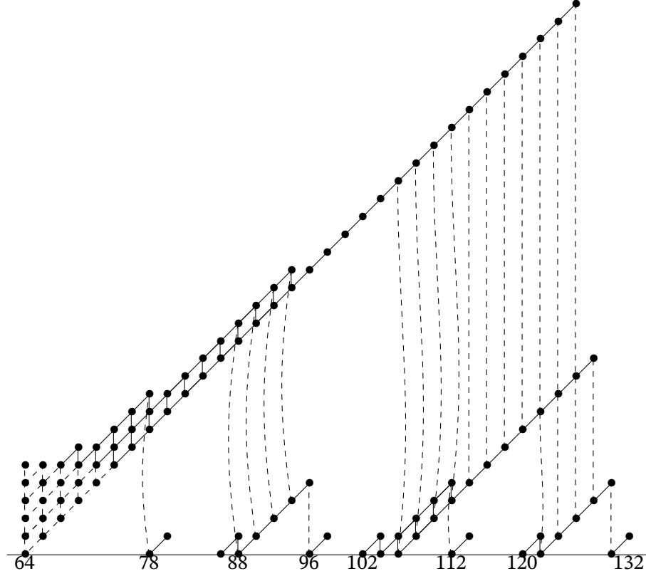
Figure 1.2. \mathcal{A}_5 , the ku -homology analogue of A_5 , from [11]
