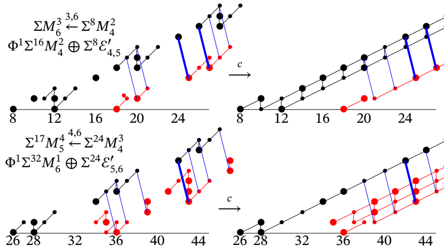
Figure 14.6. d_5 differentials (look like d_4 )
