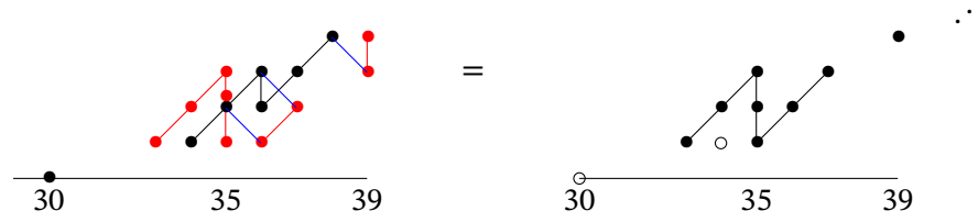
Figure 12.7. \Sigma^{25}M_4^3 \leftarrow \Sigma^{32}M_6^0
