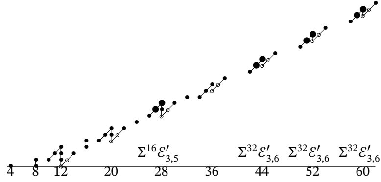
Figure 4.12. \mathcal{E}'_{2,6} and differentials
