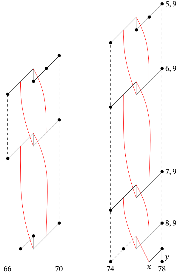
Figure 18.5. Forming the end of the 84-dual of \tilde{\mathcal{A}}_5^*
