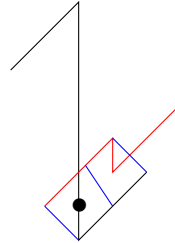
Figure 15.1. Last step in forming \Sigma^{2^{k+1}}M_{\ell-k+3}
