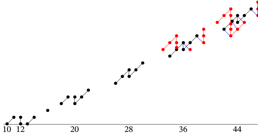
Figure 13.10. Forming \Sigma^{32}M_{t-3}^{e+5-t} \oplus \mathcal{E}'_{e,e+3}
