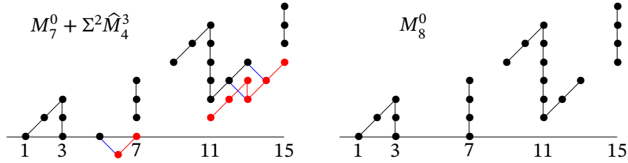
Figure 13.3. M_7^0 + \Sigma^2 \hat{M}_4^3 = M_8^0
