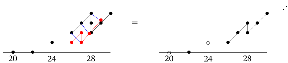
Figure 12.6. \Sigma^{17} M_5^2 \leftarrow \Sigma^{24} M_4^1
