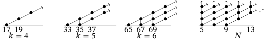
Figure 9.7. \text{Ext}_{E_1}(M_k, \mathbb{Z}_2) and \text{Ext}_{E_1}(N, \mathbb{Z}_2) .
