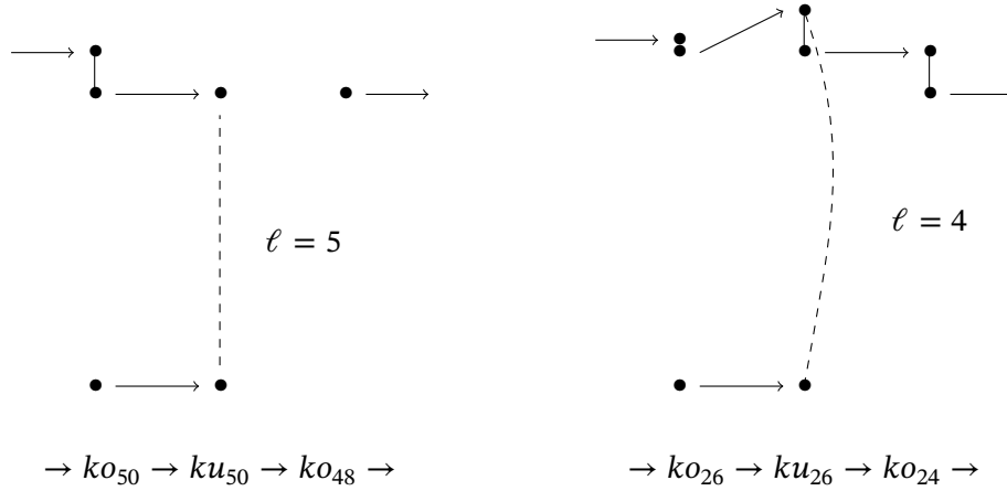
Figure 14.10. Extensions from \Sigma^{2^\ell} \mathcal{E}_{2,\ell} into \mathcal{E}_{1,5}
