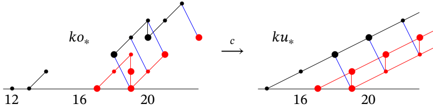
Figure 12.4. Deducing a ko differential from ku
