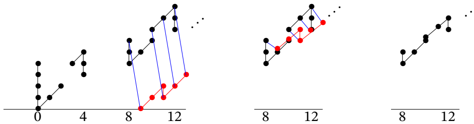
Figure 12.3. V_4 \leftarrow \Sigma^8 M_4^0
