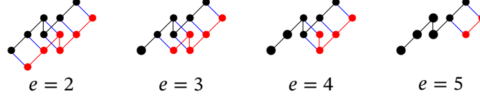
Figure 4.17. Termination of \mathcal{E}'_{e,e+d}
