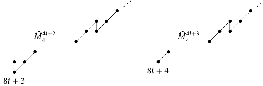
Figure 4.6. \widehat{M}_4^s for s \equiv 2, 3 \pmod{4}
