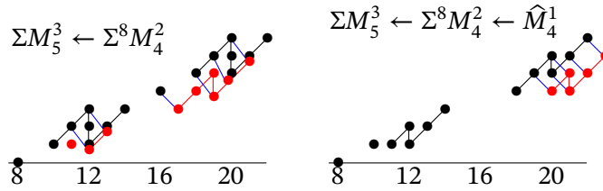
Figure 4.16. Formation of \mathcal{E}'_{3,5}
