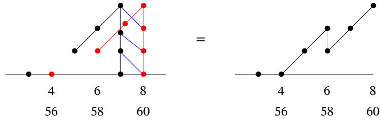
Figure 15.3. Cofiber of 2 on P_3 \wedge bo equals \Sigma^4 M \wedge bo \vee H
