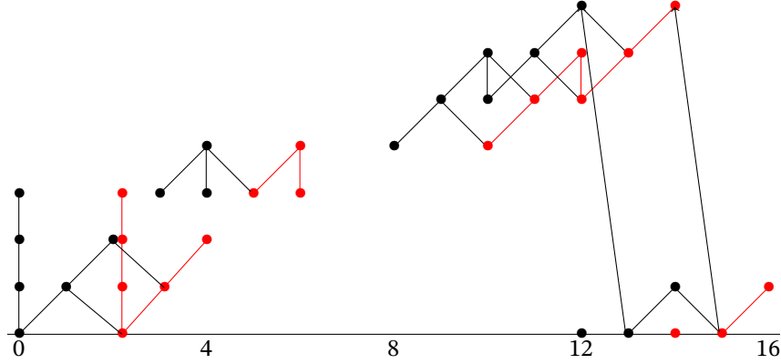
Figure 16.5. Forming \widetilde{\mathcal{A}}_3 from \widetilde{\mathcal{A}}_3 \oplus \Sigma^2 \widetilde{\mathcal{A}}_3 .
