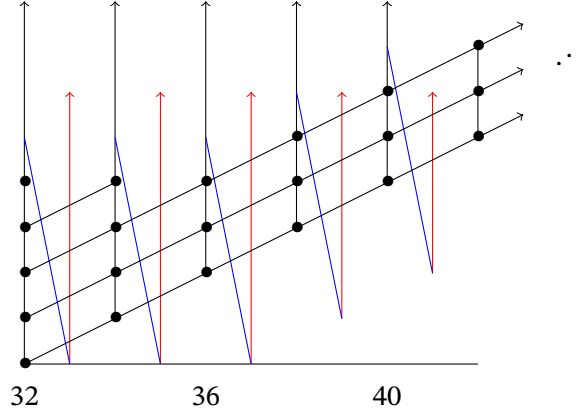
Figure 9.9. Differential killing infinite towers in \mathcal{A}_4 .
