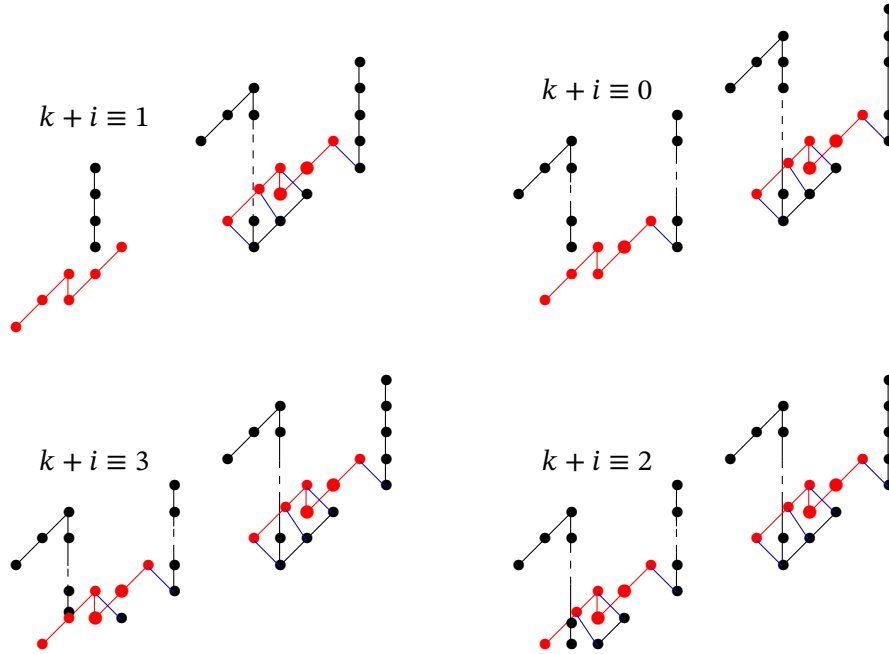
Figure 13.11. Cutting off M_k^i with lightning flashes
