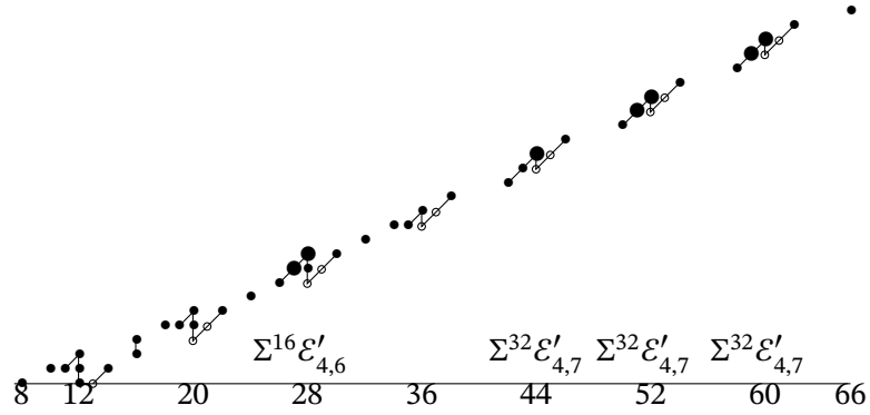
Figure 4.13. \mathcal{E}'_{3,7} and differentials
