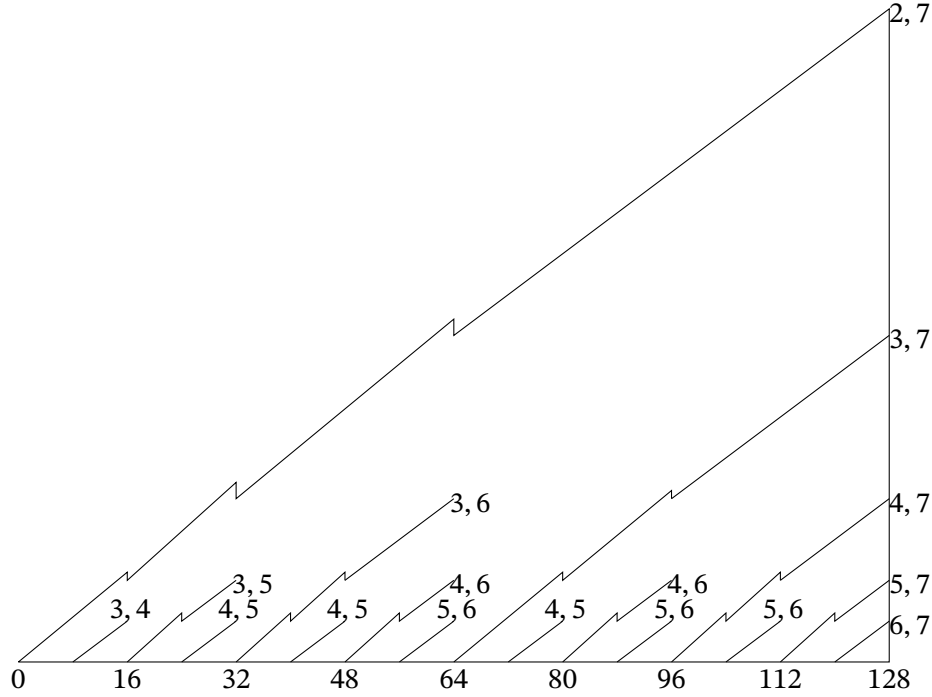
Figure 14.11. Schematic of edges under \mathcal{E}_{2,7} in grading 2 \bmod 8
