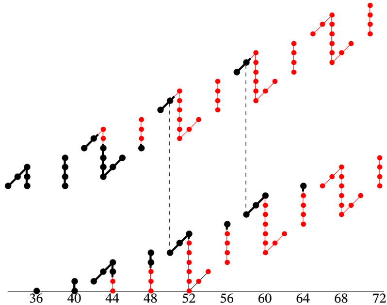
Figure 5.11. Some differentials (in red) in \widetilde{\mathcal{B}}_{4,9}
