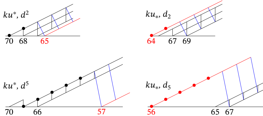
Figure 9.8. Dualizing d^2 and d^5 differentials.
