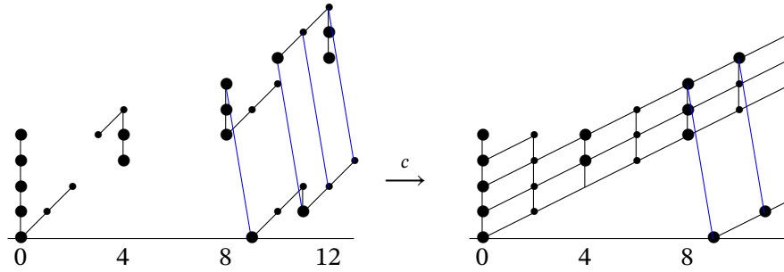
Figure 14.9. c for early part of \tilde{\mathcal{A}}_4
