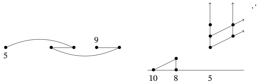
Figure 9.4. N and \text{Ext}_{E_1}(\mathbb{Z}_2, N) .
