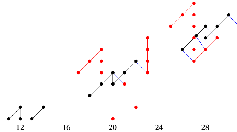
Figure 15.2. Result from first half of summands of \tilde{\mathcal{B}}_{3,7}
