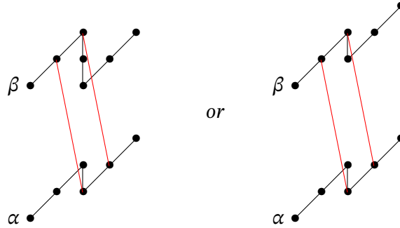
Figure 14.12. Charts implying 2\alpha = \beta
