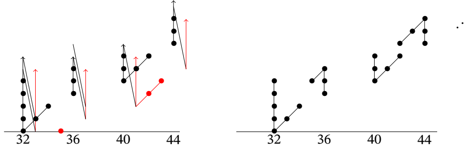
Figure 12.2. \langle y_1^8 \rangle \oplus y_1^6 NU with differentials, and redrawing.
