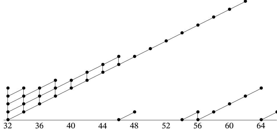
Figure 9.12. \mathcal{A}_4 without exotic extensions.
