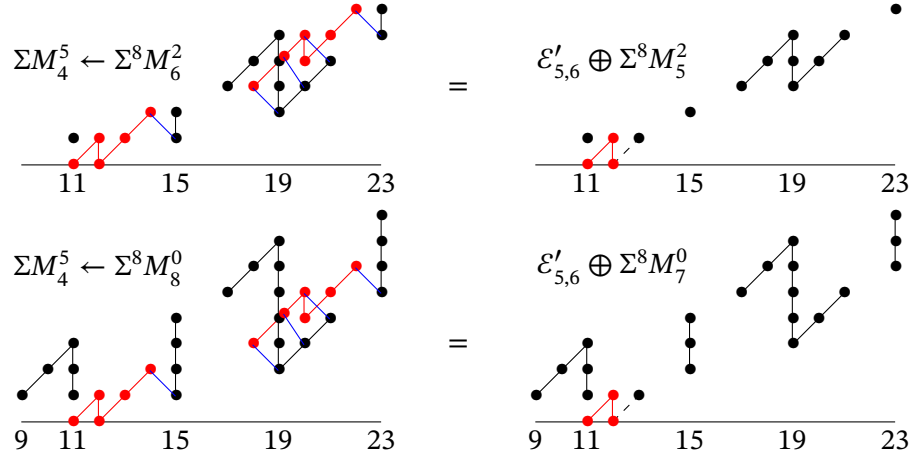
Figure 13.1. Two ways of forming \mathcal{E}'_{5,6}
