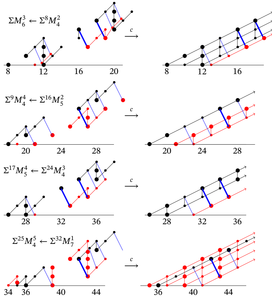
Figure 14.5. d_2 differentials ( ko_* \xrightarrow{c} ku_* )
