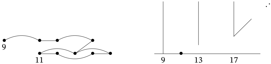
Figure 12.1. NU and its chart.
