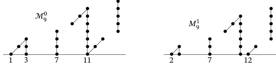
Figure 16.2. Ext charts for M_9^0 and M_9^1 .
