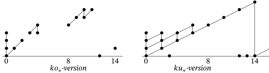
Figure 16.4. \tilde{\mathcal{A}}_3 and \tilde{\mathcal{A}}_3 .
