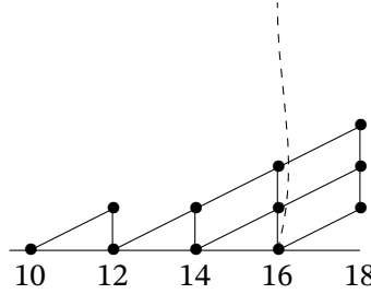
Figure 14.14. Beginning of ku analogue of \mathcal{E}_{4,k}
