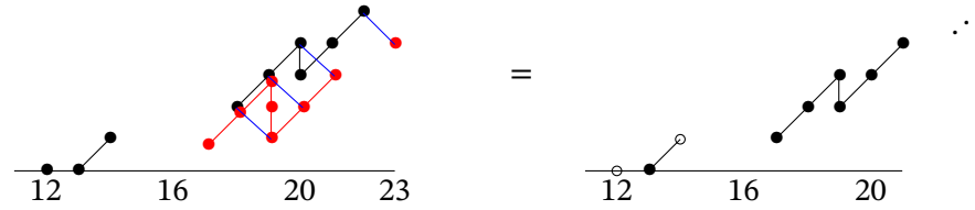
Figure 12.5. \Sigma^9 M_4^2 \leftarrow \Sigma^{16} M_5^0
