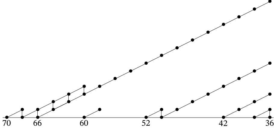
Figure 9.6. v -towers in A_4 .
