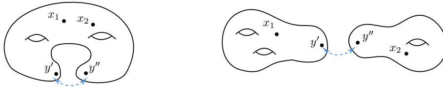
FIGURE 1. Self-sewing and disjoint sewing
