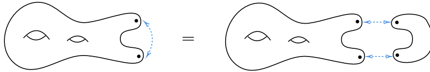
FIGURE 3. Transforming self-sewing to disjoint sewing
