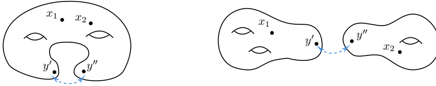
FIGURE 1. Self-sewing and disjoint sewing
