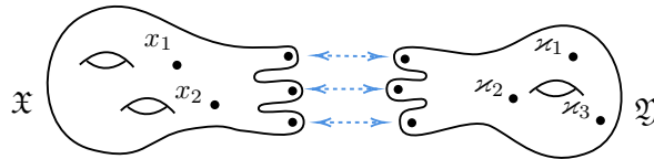
FIGURE 2. An example of \mathfrak{X} \#_{q_\bullet} \mathfrak{Y} where N = 2, K = 3, M = 3 . \mathfrak{X} \#_{q_\bullet} \mathfrak{Y} has genus-5
