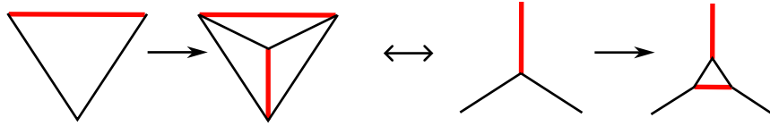
FIGURE 15. Triangle move is dual to central subdivision.
