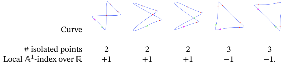
FIGURE 3. Maximally inflected real quartics, [KS03, p. 23]
