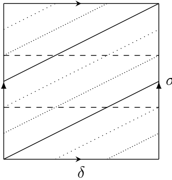
FIGURE 2. The pullback of N_{2/3}(\gamma) along f_* : D^2 \rightarrow D^2(3) is N_{2/1}(f^{-1}(\gamma)) . \delta and the dashed lines are fibers of N_{2/1} with image the same fiber in N_{2/3} , and \sigma is a section of \partial N_{2/1} . The diagonal lines are meridians of \partial N_{2/1} with the same image in N_{2/3} .
