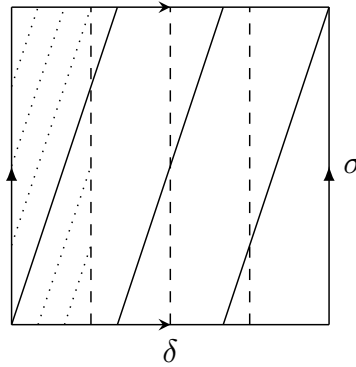
FIGURE 1. The degree 4 fiberwise quotient of N_{1/3}(\gamma) is N_{4/3}(f(\gamma)) . \delta is a fiber in N_{1/3} , \sigma and the dashed lines are sections of \partial N_{1/3} with the same image in N_{4/3} , the solid diagonal line is a meridian of N_{1/3} , and the dotted line is its image in N_{4/3} .
