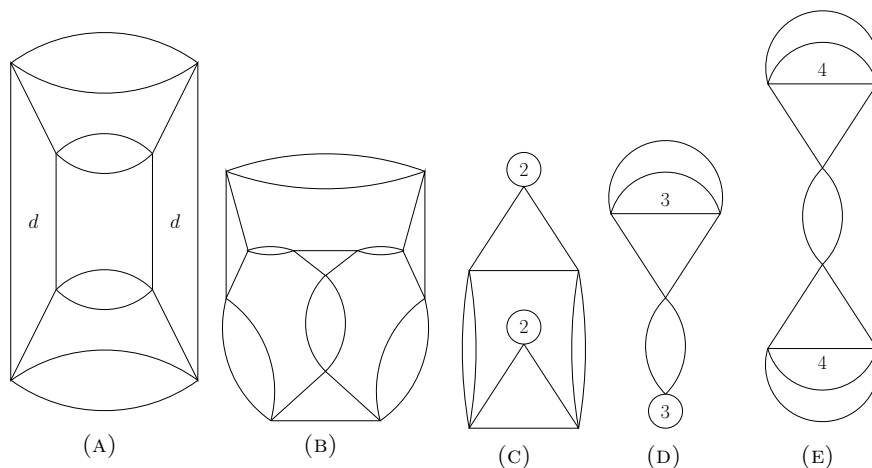
FIGURE 5. More orbifold covers from Proposition 5.5. Figure (A) is drawn for x/d = 4 . In general, d would be labeling an x/d -gon.
