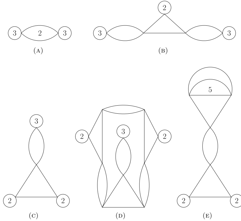
FIGURE 4. Some orbifold covers from Proposition 5.5.
