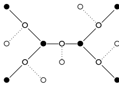
FIGURE 3. Embedded trees for \mathrm{SL}_2 (totally ramified case).
