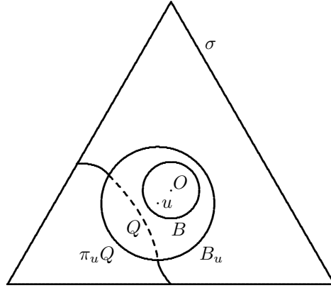
Figure 1: Projecting Q to the boundary of B_u .
