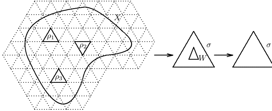
Figure 2: Making the map f simplicial
